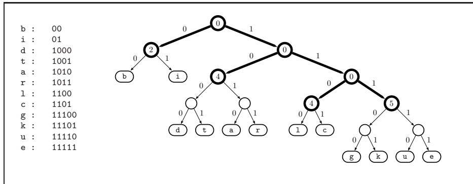
Fig. 3. The Huffman tree induced by a Huffman code for the set of symbols \Sigma = \{a, b, c, d, e, g, i, k, l, r, t, u\} . The skeleton tree is in bold.
