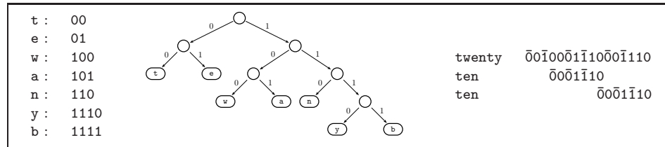
Fig. 1. A Huffman code for the set of symbols \{t, e, w, a, n, y, b\} . The binary string \bar{0}0\bar{1}00\bar{0}1\bar{1}10\bar{0}0\bar{1}110 is the encoding of the string twenty , where a “bar” indicates the starting bit of each codeword. Two occurrences of the binary string ten start at the 4-th and 10-th bit of the encoded version of the string twenty . Both of them are false matches.
