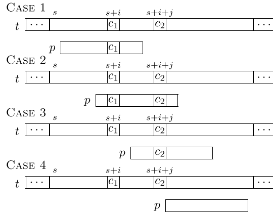
Fig. 4. The four cases of the generalized double occurrence heuristic. In Case 1 only character c_1 is involved in the computation of the shift advancement. In Case 2 both characters c_1 and c_2 occur in the pattern p , whereas in Case 3 only character c_2 is involved in the shift. Finally, Case 4 corresponds to a maximal shift advancement.
