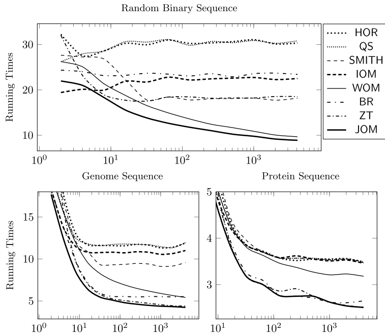
Fig. 7. Running times obtained by comparing several efficient algorithms based on the occurrence heuristic shifting strategy. The x-axis represents length of patterns.
