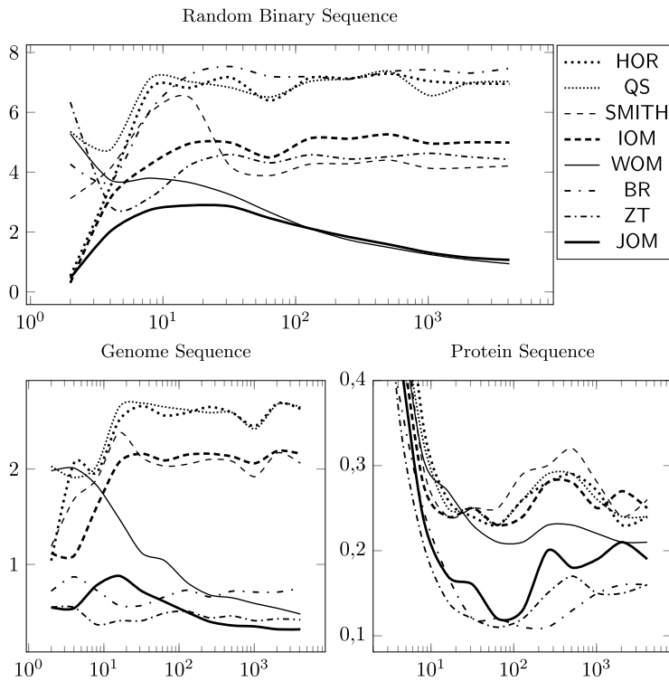
Fig. 8. Standard Deviation of running times obtained by comparing several efficient algorithms based on the occurrence heuristic shifting strategy. The x-axis represents length of patterns.
