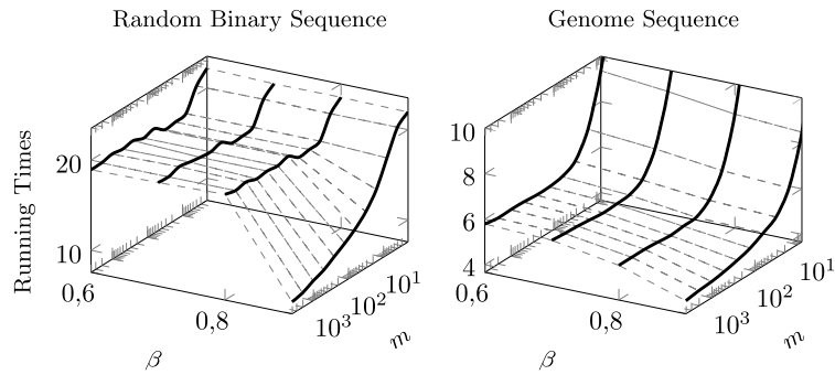
Fig. 6. Running times of the Jumping-Occurrence Matcher for different values of the parameter \beta and pattern length m .
