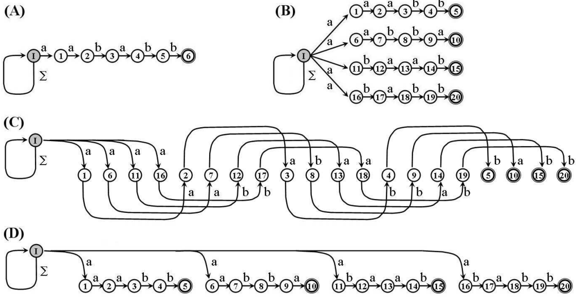
Figure 1: (A) A NFA which recognizes the pattern P = aababb . (B) A NFA obtained by the maximal trie \mathcal{T} of the set of patterns \mathcal{P} = \{aaabb, aabba, abaab, ababb\} . (C) The parallel topological ordering of \mathcal{T} . (D) The sequential topological ordering of \mathcal{T} .
