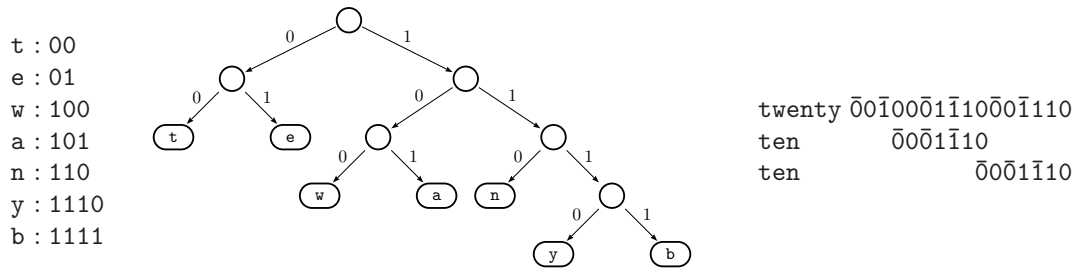
Figure 1. A Huffman code for the set of symbols {t, e, w, a, n, y, b}. The binary string \bar{0}0\bar{1}00\bar{0}1\bar{1}10\bar{0}0\bar{1}110 is the encoding of the string twenty , where a “bar” indicates the starting bit of each codeword. Two occurrences of the binary string ten start at the 4-th and 10-th bit of the encoded version of the string twenty . Both of them are false matches.
