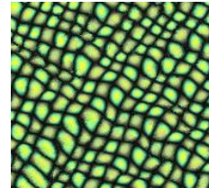
Synthetic
