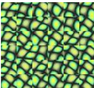
Computer Vision
